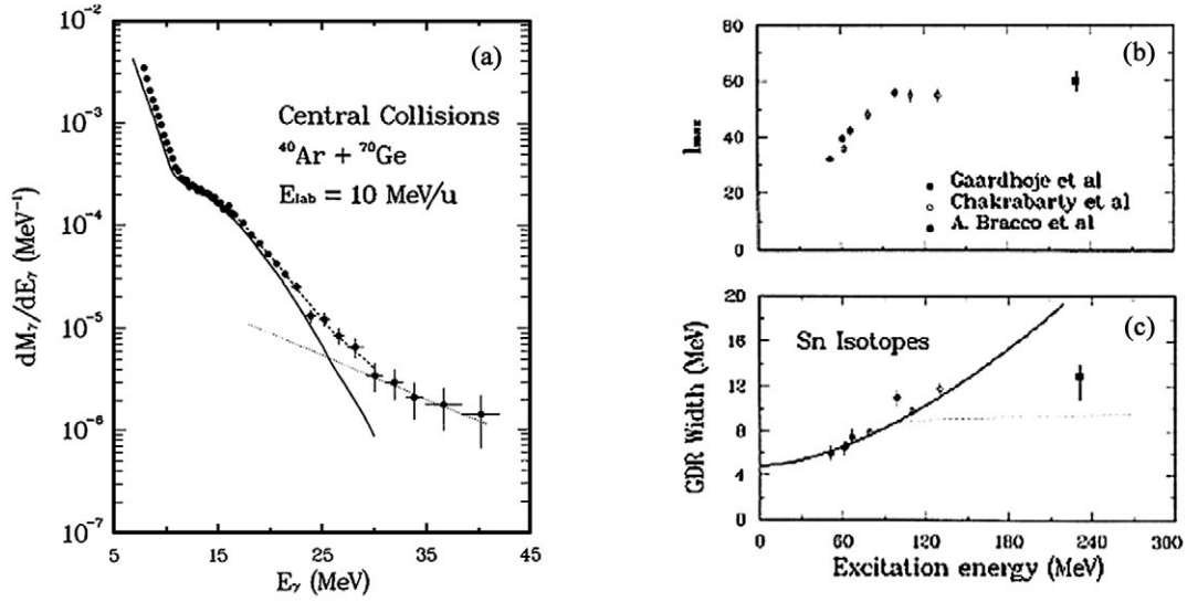
Fig. 3. a) Gamma spectrum measured in coincidence with fusion events from the reaction ^{40}\text{Ar} + ^{70}\text{Ge} at E_{\text{lab}} = 10 \text{ A MeV} . Full line represents the statistical calculation, the dotted line indicates the bremsstrahlung contribution while the dashed line is the sum of the previous two. b) The trend of the maximum angular momentum populated in the different fusion reactions leading to Sn isotopes as a function of excitation energy. c) The systematics of the GDR width measured on ^{108-112}\text{Sn} isotopes as a function of excitation energy. The width value at E^* = 230 \text{ MeV} is the one measured by Bracco et al. [16] suggesting the width saturation. The full line corresponds to the parametrization of the width given by eq.6.
