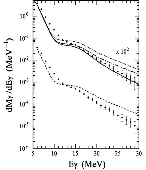
Fig. 16. Top: Comparison between spectra extracted at 500 MeV excitation energy in the reaction ^{36}\text{Ar} + ^{90}\text{Zr} @ 27A MeV [52] with statistical calculations including models prescriptions of Bortignon et al. [38] (solid line), Smerzi et al. [41] (dot-dashed line) and Chomaz [40] (dotted line). Bottom: Same spectrum compared with the prediction of statistical calculation including a width increasing with E^* according to eq.6 shown as a dashed line
