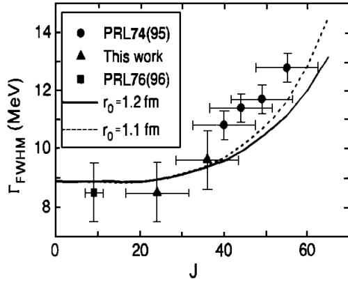
Fig. 5. Evolution of the width as a function of angular momentum at T \sim 2 MeV [20]. The solid line represents a calculation of the width evolution with spin assuming a moment of inertia of the nucleus equal to the rigid rotor value while the dashed line is a similar calculation assuming a reduction of 16% in the rigid rotor value [20].
