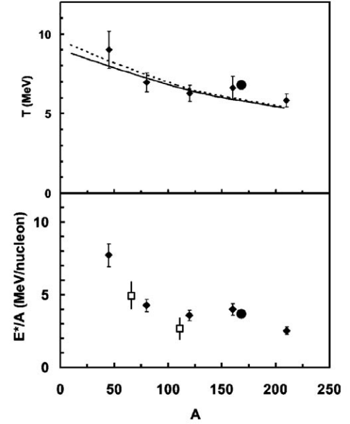
Fig. 20. Top panel shows the dependence of the limiting temperature (of the plateau of the caloric curves) on the mass of the system. Bottom panel shows the excitation energy per nucleon at which the limiting temperature is reached as a function of the system mass [69]. Open symbols are the limiting excitation energies per nucleon for the GDR for two mass regions.
