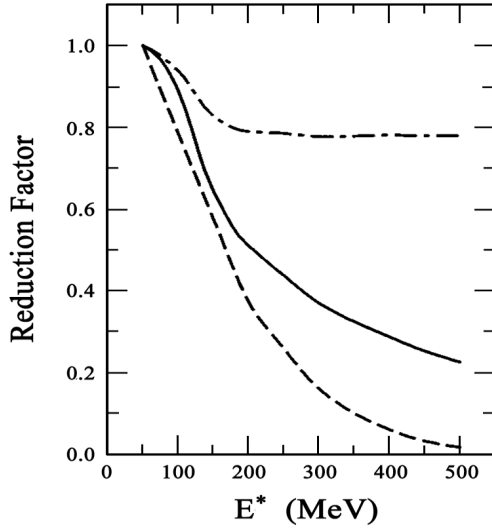
Fig. 17. Predictions of GDR quenching factor as a function of E^* [52] according to the models of Bortignon et al. [38] (solid line), Smerzi et al. [41] (dot-dashed line) and Chomaz [40] (dashed line).
