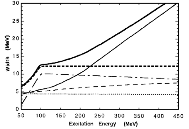
Fig. 12. Evolution of the total GDR width and its various components in Sn isotopes as a function of excitation energy. The thick solid line displays the total width predictions according to the parametrization suggested in ref.[45] including the particle evaporation width contribution [44]. The thick dashed line represents the standard prediction assuming the saturation at 12 MeV. The thin lines show the contribution to the width due to the various components. In particular, the thin solid line represents the intrinsic width including the particle evaporation width contribution while the dotted one shows the intrinsic width.
