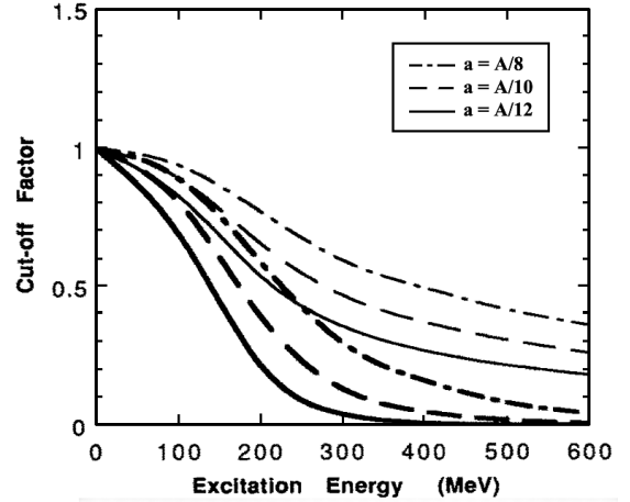
Fig. 10. Evolution of quenching factors predicted for Sn nuclei as a function of excitation energy for different values of the level density parameter. Thick lines show the reduction factor predicted in ref.[38] while thin lines are predictions made according to ref.[40]
