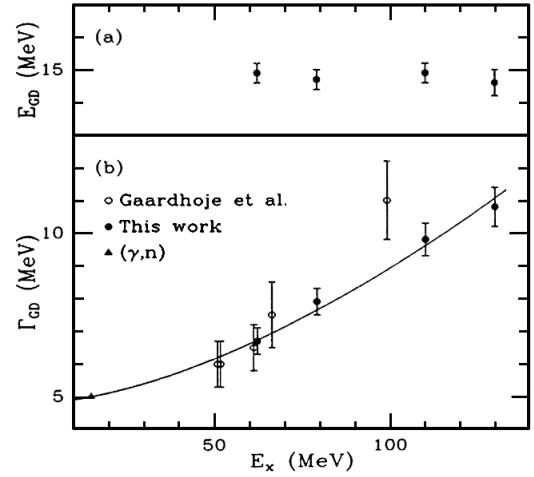
Fig. 2. The systematics for the energy (a) and width (b) as a function of E^* . Open symbols are from ref.[13,14] while full symbols are from ref. [15]. The full line corresponds to the parametrization of the width given by eq.6.
