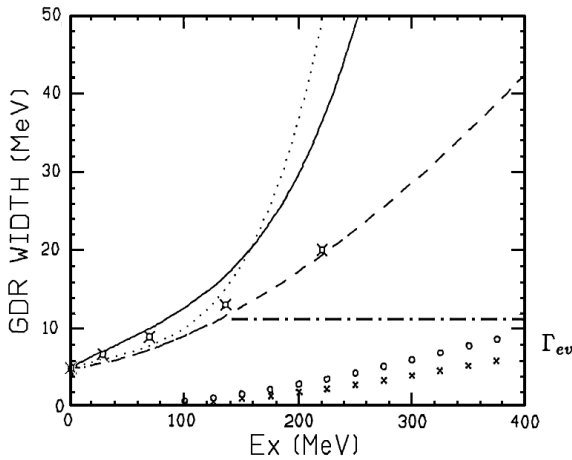
Fig. 11. Excitation energy dependence of the GDR width for Sn isotopes. Open square symbols represent the results of the calculations of Bonasera et al.[43]. The dashed line is the extrapolation to higher energies of the width parametrization given by eq.6. The solid line is a previous estimate for the width increase [41], the dotted one is a fit of the width trend extracted from ref. [46] and the dot-dashed one is a parametrization assuming a constant width of 11 MeV above E^* = 130 MeV. In the same figure the \Gamma_{ev} values calculated for level density parameters a = A/12 (circles) and a = A/10 (crosses) are shown.
