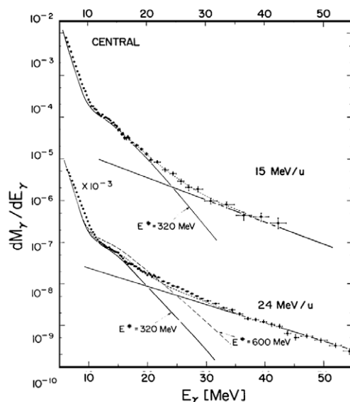
Fig. 7. Gamma spectra measured in the reactions ^{40}\text{Ar} + ^{70}\text{Ge} at 15 and 24A MeV. Full line represents the statistical model calculation performed at E^* = 320 MeV while the dashed line is a calculation assuming E^* = 600 MeV. Dotted lines are the sum of statistical plus bremsstrahlung contributions. [36].
