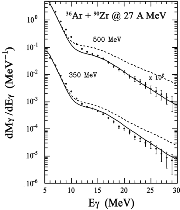
Fig. 15. Comparison of the gamma spectra extracted for 350 and 500 MeV excitation energy bins after bremsstrahlung subtraction with statistical calculations [52]. Dashed line represents the standard calculation while the full line is a calculation including the suppression of the GDR emission above E^* = 250 MeV.
