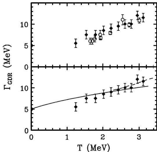
Fig. 4. Comparison of the GDR width extracted from 50A MeV \alpha -particle inelastic scattering experiment (full symbols) on ^{120}\text{Sn} [19] and from fusion reaction data (open symbols) on ^{108-112}\text{Sn} nuclei [13–15]. The lower part shows the comparison of the \alpha inelastic scattering experiment results with adiabatic coupling calculations [22] shown as a full line. The dashed line includes the contribution to the width due to particle evaporation width [44].
