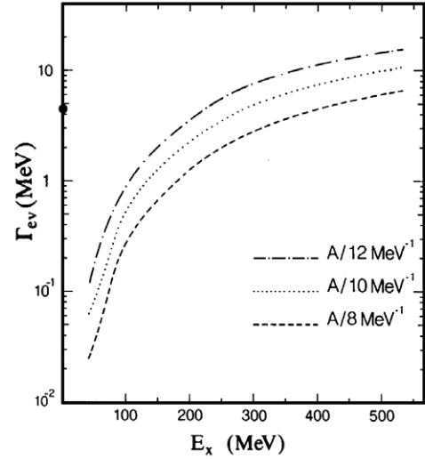
Fig. 8. Particle evaporation widths as a function of excitation energy estimated in the framework of statistical model for three values of the level density parameter ranging from a = A/8 to a = A/12 [38]. The full symbol represents the value of the \Gamma^\downarrow of the GDR measured on the ground state in ^{108}\text{Sn}
