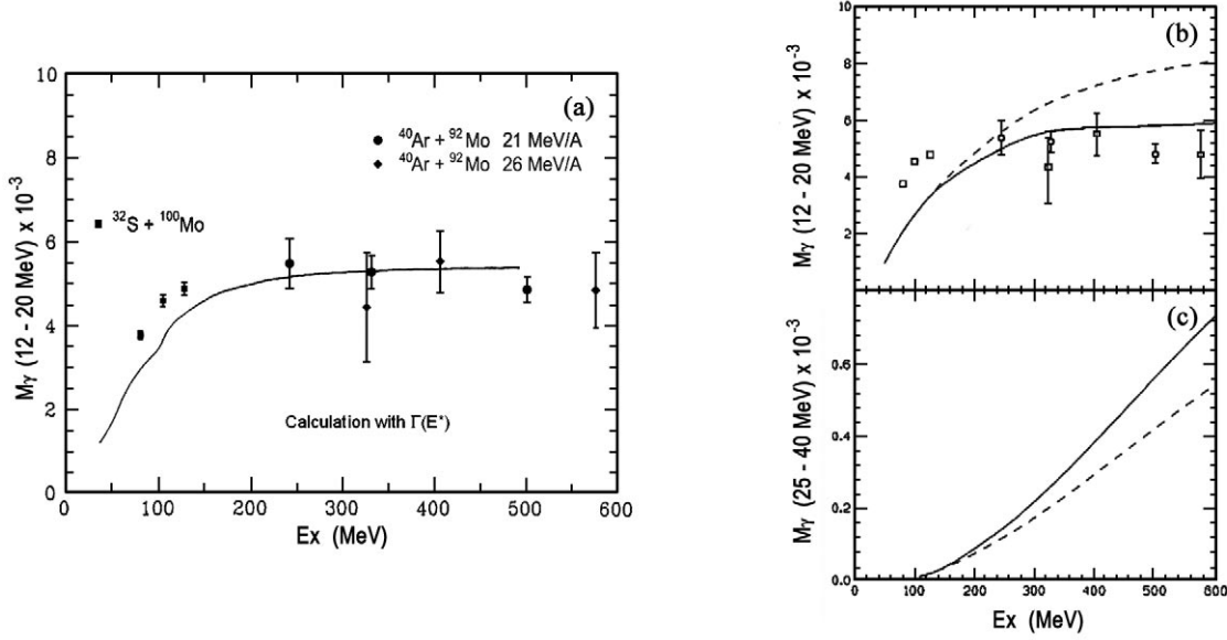
Fig. 13. a) Evolution of the gamma yield integrated in the region between 12 and 20 MeV as a function of excitation energy for different reactions. Circles correspond to 21A MeV data, diamonds to 26A MeV data while squares are from the reaction ^{32}\text{S} + ^{100}\text{Mo} @ 150, 180 and 210 MeV beam energies [47]. The solid line represents the calculation of the \gamma yield, integrated in the same energy region, according to the parametrization adopted in ref.[46]. b) Comparison between the same set of data and the theoretical predictions according to Smerzi et al. [42], (solid line) and Bortignon et al. [38] (dashed line) c) Same model calculation as above but in the energy region 25 - 40 MeV.
