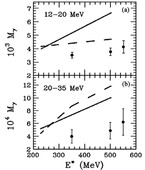
Fig. 14. a) Evolution of the gamma yield integrated in the region between 12 and 20 MeV as a function of excitation energy for the reaction ^{36}\text{Ar} + ^{90}\text{Zr} @ 27 A MeV [52]. Full symbols are experimental results, full line is prediction of the standard statistical calculation while the dashed one is the prediction of statistical calculation including a parametrization for the width given by eq.6 [52, 15]. b) Same comparison as above but in the energy region 20–35 MeV.
