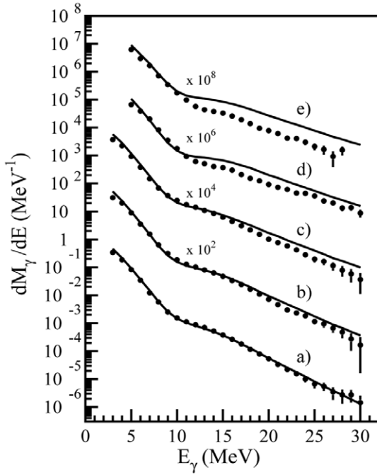
Fig. 18. Gamma-ray spectra measured at 160, 200, 290, 350 and 430 MeV excitation energy (a-e) in coincidence with evaporation residues. The spectra at E^* = 160 and 200 MeV are from the reactions ^{116}\text{Sn} + ^{12}\text{C} @ 17 and 23A MeV, the one at E^* = 290 MeV is from the reaction ^{116}\text{Sn} + ^{24}\text{Mg} @ 17A MeV while the spectra at higher excitation energies were measured in the reaction ^{36}\text{Ar} + ^{98}\text{Mo} @ 37A MeV. Solid lines represent the corresponding Cascade calculations performed assuming 100% of the EWSR and a constant width \Gamma = 12 MeV.
