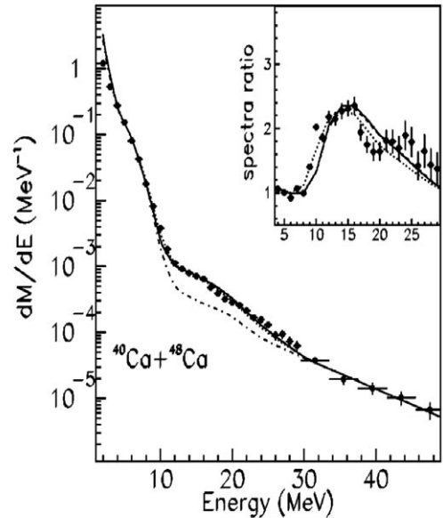
Fig. 19. Gamma-ray spectrum measured in the reaction ^{40}\text{Ca} + ^{48}\text{Ca} @ 25A MeV in coincidence with evaporation residues. The full line is a calculation assuming a cut-off energy for the GDR emission at E^* = 260 MeV and a width \Gamma = 15 MeV. The dashed line is a calculation assuming a smooth cut-off expression according to [38]. The dotted line is instead obtained assuming again a cut-off energy at E^* = 260 MeV but a mass A = 70 for the emitting system. The dot-dashed line is a GDR zero strength calculation used to linearize the experimental data and calculations shown in the inset.
