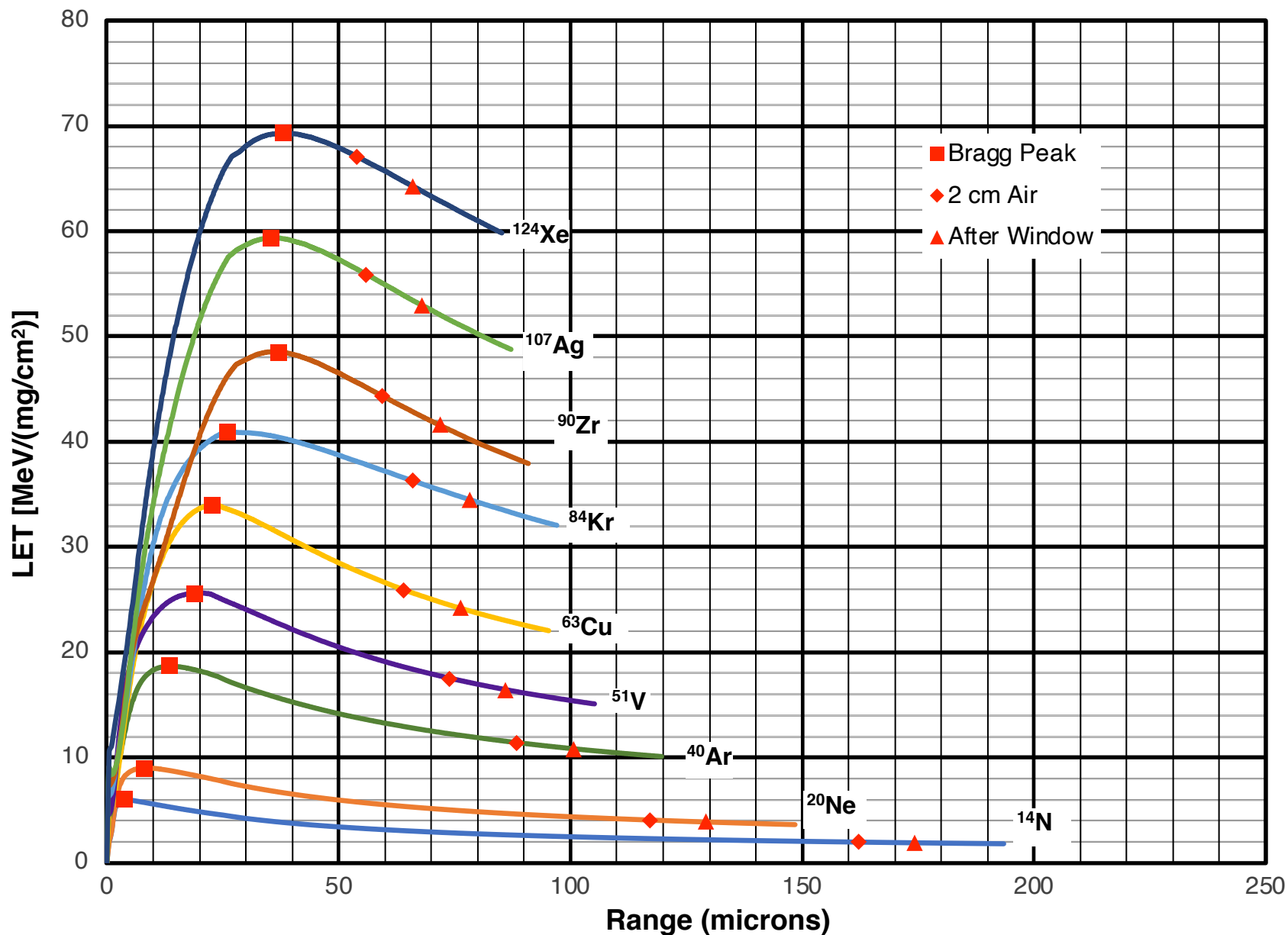
LET vs Range in Silicon for 9.4 MeV/u K150 Beams
