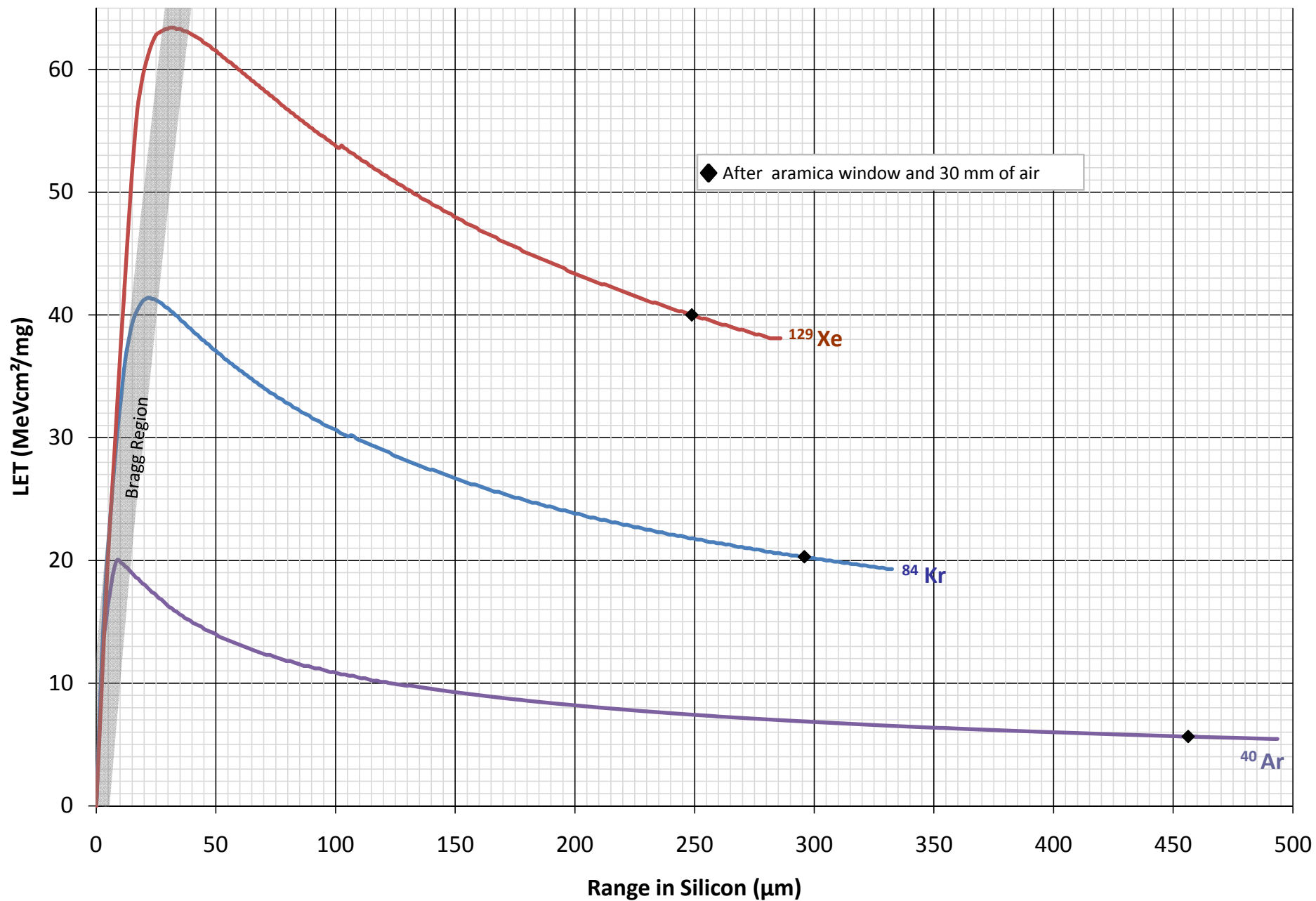
LET vs. Range in Si for 25 MeV SEE Beams
