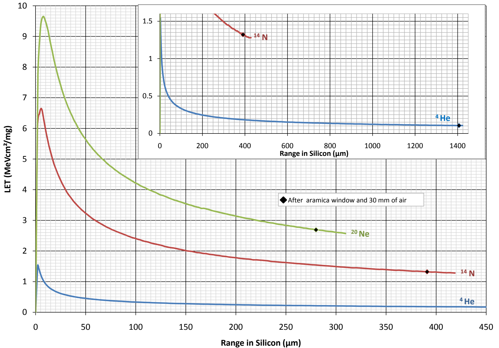
LET vs. Range in Si for 15 MeV SEE Beams (low LET)
